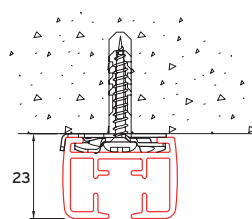
ceiling fixing with clamp 6050
