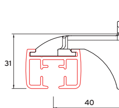
wall fixing with support 6051
